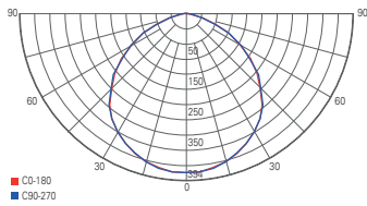
light distribution curve 732043
