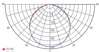
light distribution curve 565320, 565367
