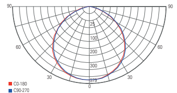
light distribution curve 732140
