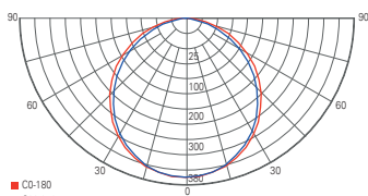
light distribution curve 565323, 565370
