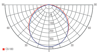
light distribution curve 565321, 565368
