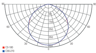
light distribution curve 732045
