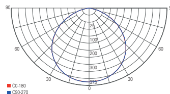
light distribution curve 732142
