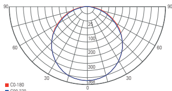
light distribution curve 565322, 565369
