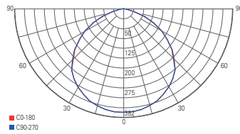
light distribution curve 732097
