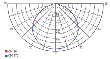
light distribution curve 732099
